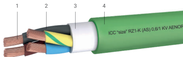
1. Rame flessibile Classe 5 IEC 60228 | Flexible copper Class 5 IEC 60228 2. XLPE DIX 3 | XLPE DIX 3. Riempitivo | Extruded filler 4. Termoplastico DMZ-E-LSOH | Thermoplastic DMZ-E-LSOH
