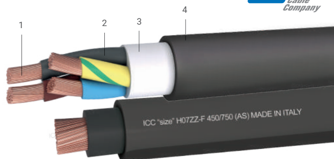
1. Rame flessibile classe 5 CEI EN 60228 | 1. Flexible bare copper class 5 CEI EN 60228 • 2. Gomma E18 LSOH | 2. Rubber E18 LSOH • 3. Riempitivo gomma LSOH (size over 6 mm 2 ) | 3. LSOH Rubber filler (size over 6 mm 2 ) • 4. Gomma EM8 LSOH | 4. Rubber EM8 LSOH
